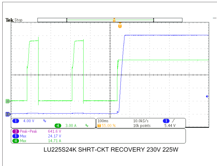
Fig. 24: SHORT-CIRCUIT AT 230VAC 24V 9.38A – CH4: 3A Div.
