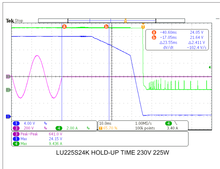
Fig. 15: HOLD-UP TIME AT 230VAC 24V 9.38A – CH4: 2A Div.
