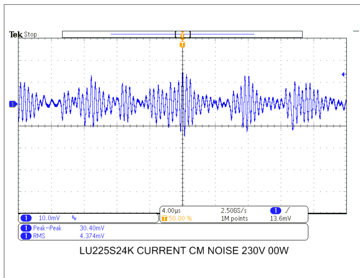
Fig. 27: CM NOISE CURRENT AT 230VAC 24V 0A – CH1 1mA/1mV
