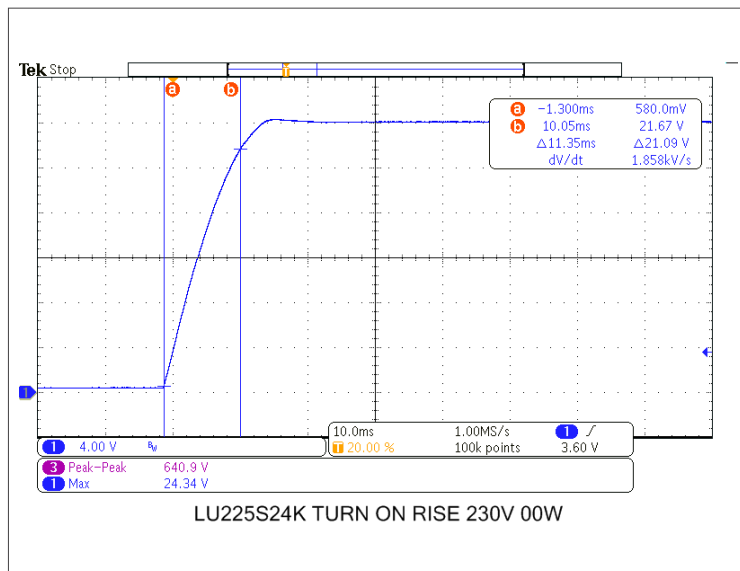
Fig. 9: TURN-ON RISE TIME AT 230VAC 24V 0A
