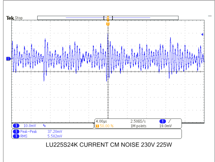
Fig. 30: CM NOISE VOLTAGE AT 230VAC 24V 9.38A – CH1 1mA/1mV
