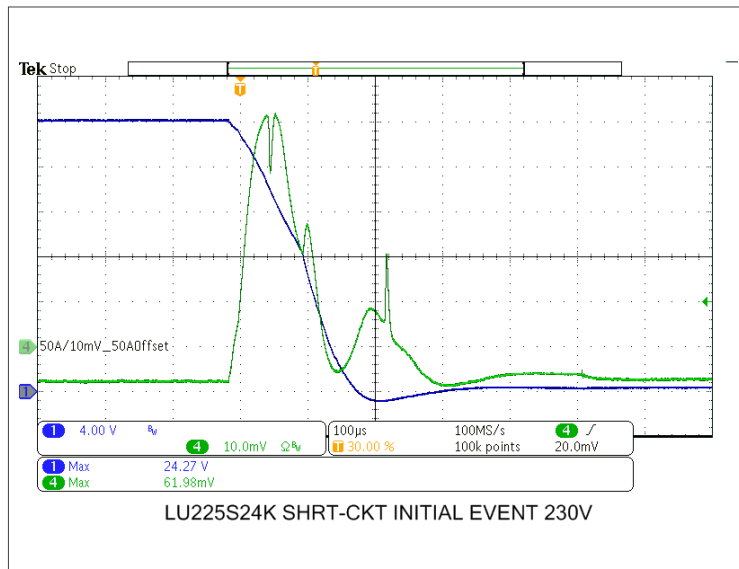
Fig. 21: SHORT-CIRCUIT AT 230VAC 24V 9.38A – CH4: 50A Div.
