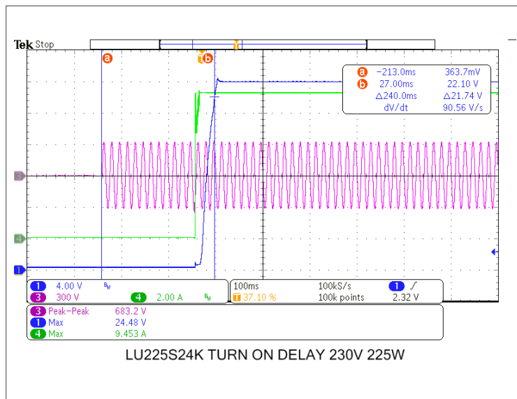
Fig. 6: TURN-ON DELAY AT 230VAC 24V 9.38A – CH4: 2A Div.
