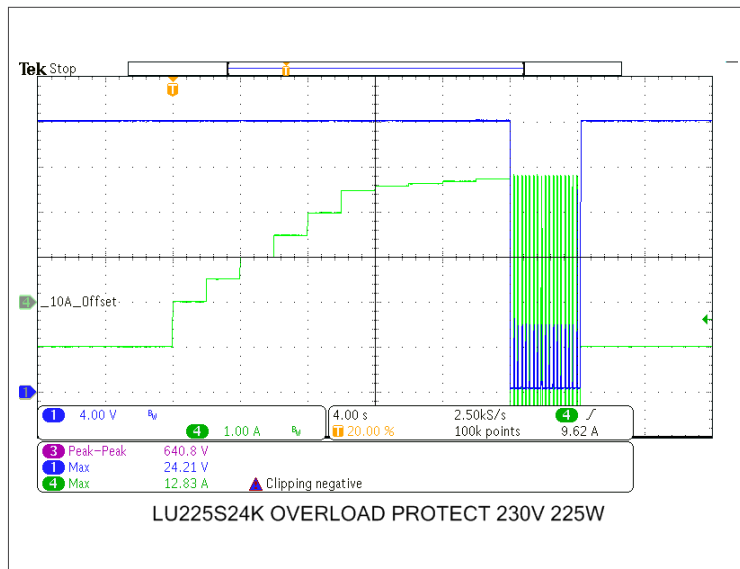
Fig. 18: OVERLOAD AT 230VAC 24V 9.38A – CH4: 1A Div.
