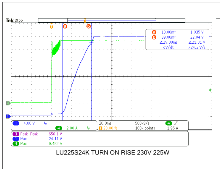
Fig. 12: TURN-ON RISE TIME AT 230VAC 24V 9.38A – CH4: 2A Div.
