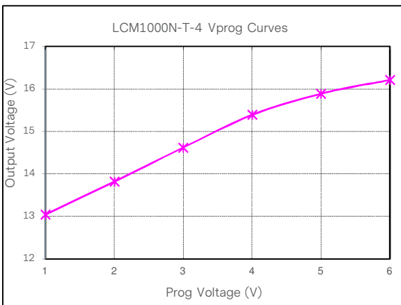
Figure 22: LCM1000N-T-4 Output Voltage Adjustment by Vprog @ 25°C Loading: Io = 0A (15V)
