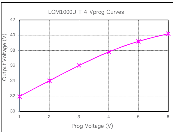
Figure 44: LCM1000U-T-4 Output Voltage Adjustment by Vprog @ 25°C Loading: Io = 0A (36V)
