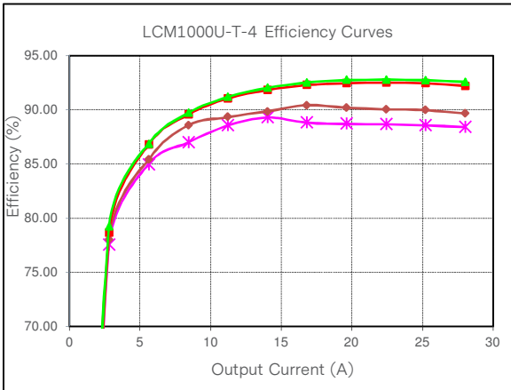
Figure 42: LCM1000U-T-4 Efficiency Curve @ 25°C Loading: Io_main = 10%Io_max increment to 27.8A
